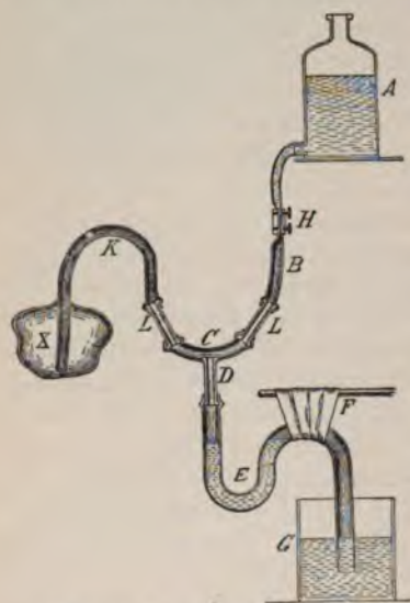
Fig. 700.—Keen's modification of Cathcart's siphonage apparatus: X, Cavity to be drained; A, reservoir; K, tube from cavity; B, tube from reservoir; H, clamp on tube from reservoir; L, L, D, glass tubes; C, rubber tube connecting cavity-drain with reservoir-drain; E, S-shaped rubber tube maintained in shape by hooking up at F; G, vessel containing antiseptic fluid.
